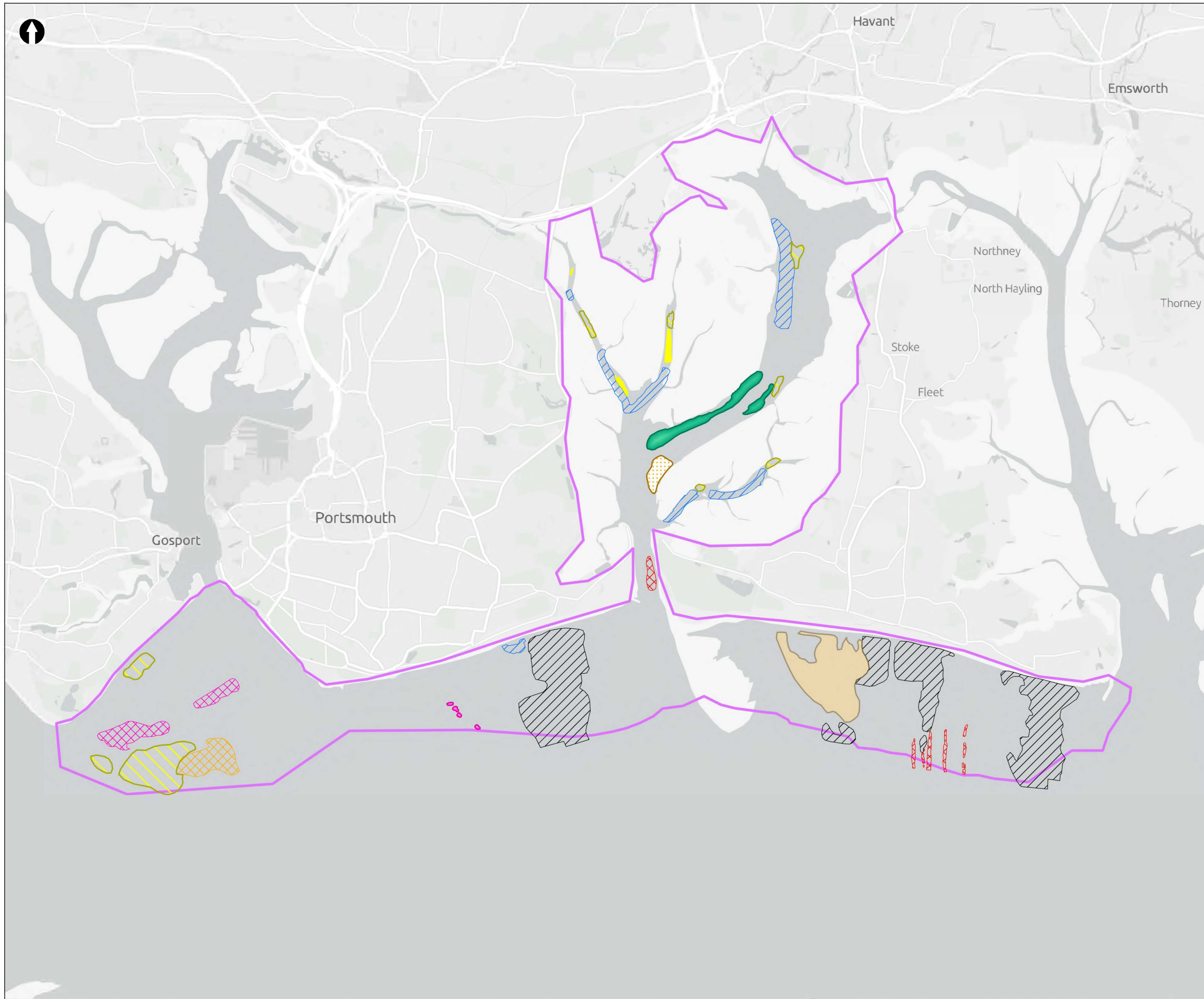
Figure 9.5 Habitat mosaic surveyed by sidescan across Longstone Harbour, south of Hayling Island and south of Eostney
